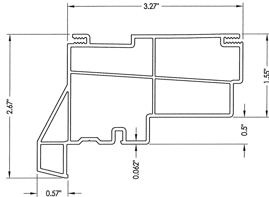
1 FRAME
